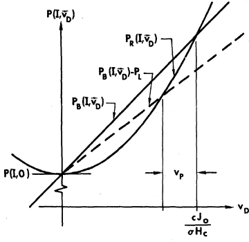
FIG. 3. The power supplied to the sample in the intermediate state by the battery P_B(I, \vec{v}_D) and the power dissipated resistively in the normal regions P_R(I, \vec{v}_D) as functions of the domain velocity \vec{v}_D [Eqs. (6) and (7)]. In the absence of pinning, energy conservation requires that P_B(I, \vec{v}_D) = P_R(I, \vec{v}_D) . Thus, solutions for v_D occur at v_D = 0 and v_D = cJ_0/\sigma H_c . With pinning, additional energy is dissipated at a rate P_L so energy conservation requires that P_B(I, \vec{v}_D) - P_L = P_R(I, \vec{v}_D) . The dashed line illustrates the left-hand side of this equation when P_L \propto \vec{v}_D . The solutions occur for v_D = 0 and v_D = cJ_0/\sigma H_c - v_p , where v_p is the decrease in the domain velocity due to pinning [Eq. (8)].
